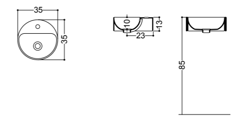
ART. WS105 03C lavabo Ø 35 da appoggio monoforo 03C overtop basin Ø 35 1/hole
