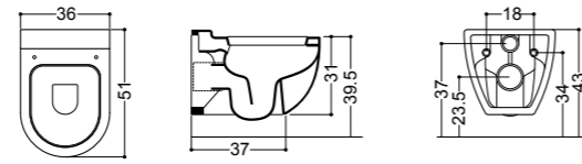
ART. 14010 vaso sospeso wall-hung wc
