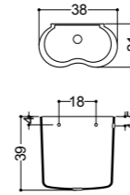
ART. 06052 cassetta a zaino low level cistern
