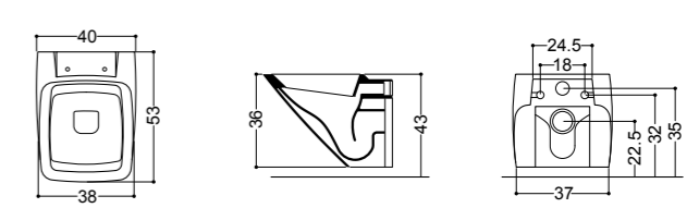
ART. 24010 vaso sospeso wall-hung wc
