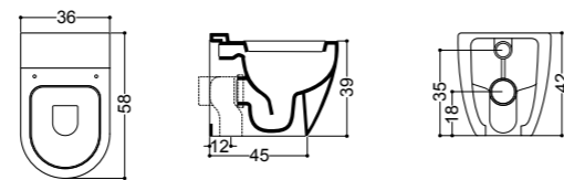
ART. 25011 vaso 58 BTW wc 58
