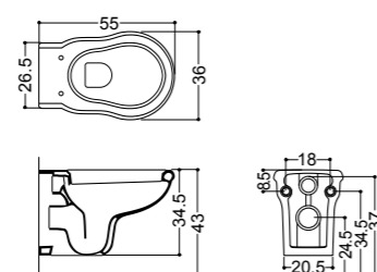
ART. 06060 vaso sospeso wall-hung wc
