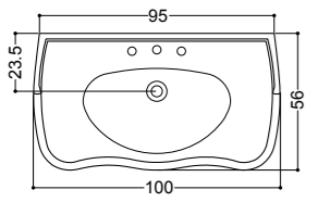
ART. 06041 gamba in ceramica ceramic leg
