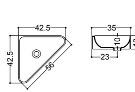
ART. WS108 04S lavabo 42 da appoggio senza piano rubinetteria 04S overtop basin 42 without tap hole
