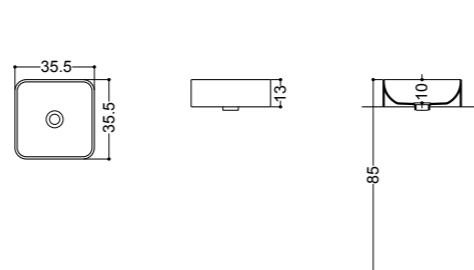
ART. WS104 02S lavabo 35 da appoggio senza piano rubinetteria 02S overtop basin 35 without tap hole
