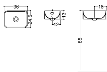
ART. WS102 01S lavabo da appoggio senza piano rubinetteria 01S overtop basin without tap hole
